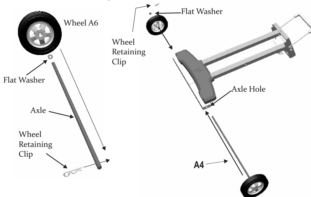
Wheel shown properly installed.
